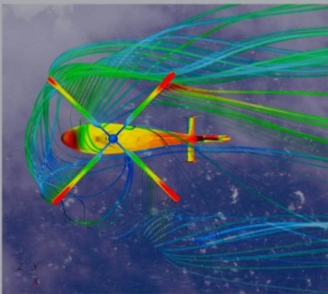
High-Rotor Noise
