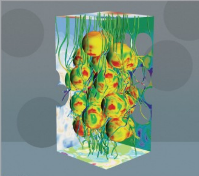
Flow through randomly stacked nuclear pebbles
